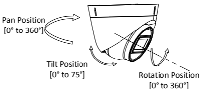
Figure 2-5 3-Axis Adjustment
