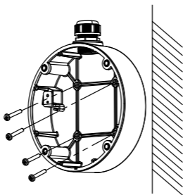
Figure 2-7 Secure the Junction Box on the Wall
