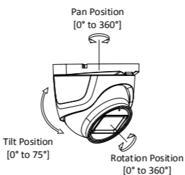
Figure 2-20 3-Axis Adjustment
